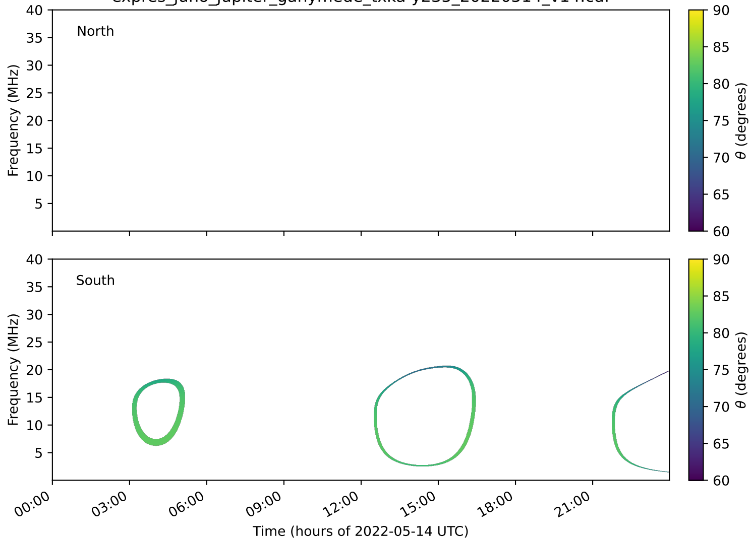
expres_juno_jupiter_ganymede_txka-y235_20220514_v14.cdf
