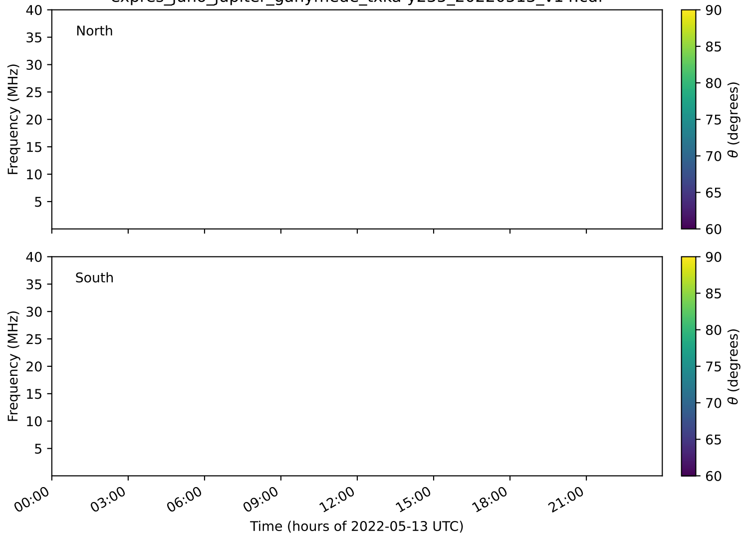
expres_juno_jupiter_ganymede_txka-y235_20220513_v14.cdf
