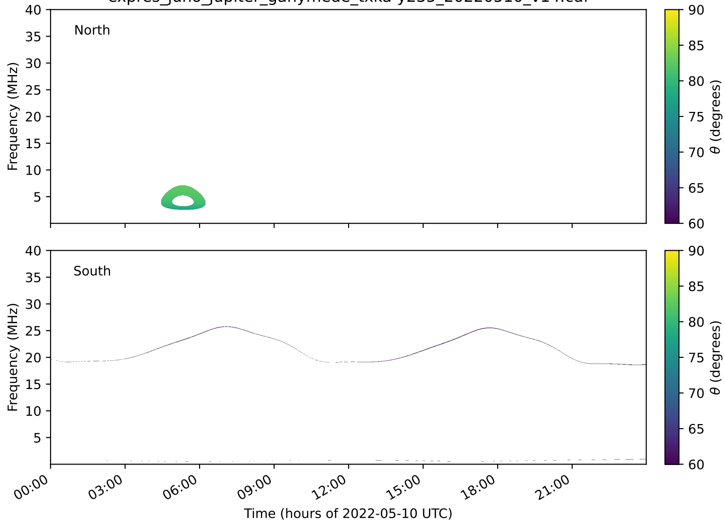
expres_juno_jupiter_ganymede_txka-y235_20220510_v14.cdf
