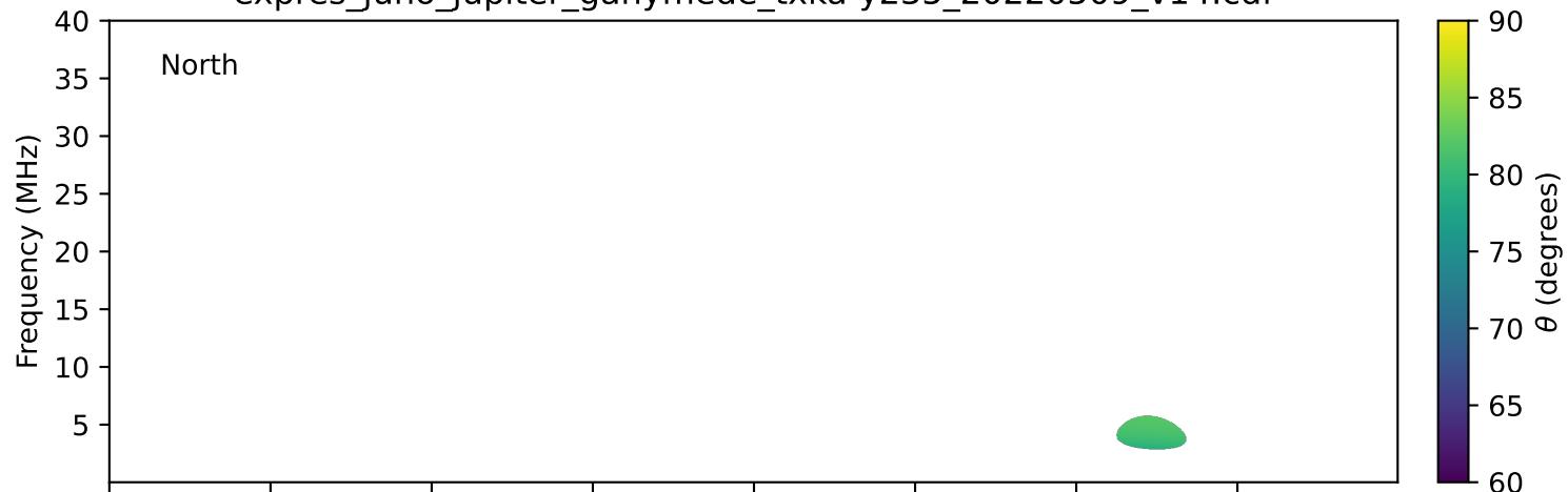
expres_juno_jupiter_ganymede_txka-y235_20220509_v14.cdf
