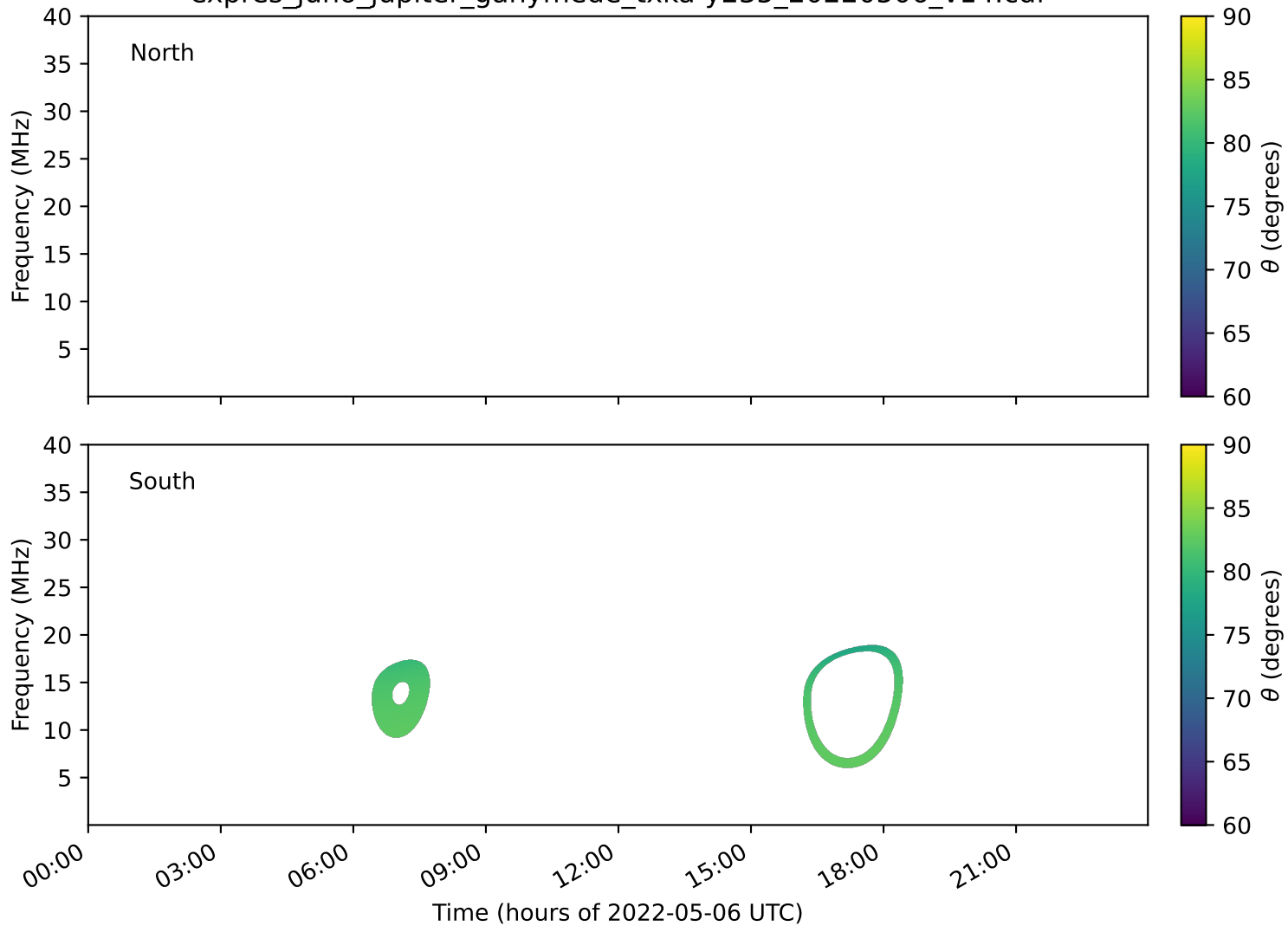
expres_juno_jupiter_ganymede_txka-y235_20220506_v14.cdf
