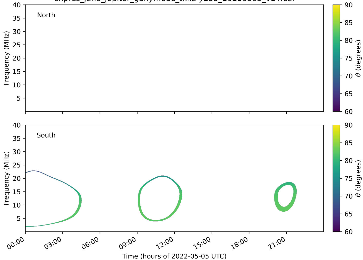
expres_juno_jupiter_ganymede_txka-y235_20220505_v14.cdf
