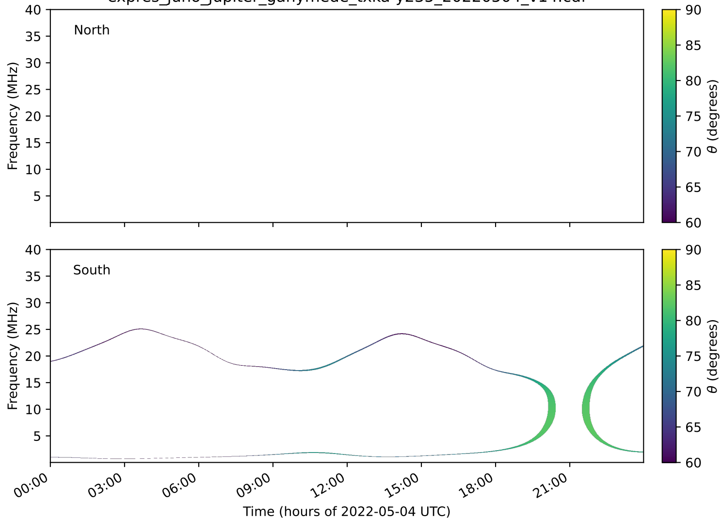
expres_juno_jupiter_ganymede_txka-y235_20220504_v14.cdf
