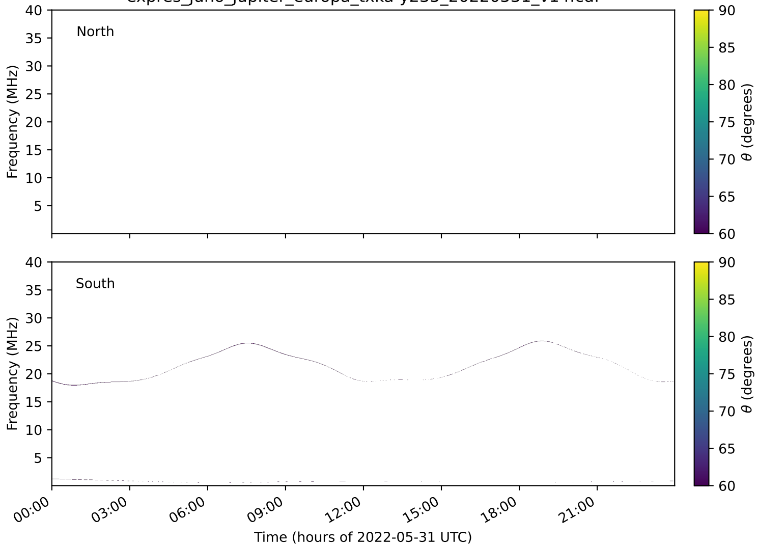
expres_juno_jupiter_europa_txka-y235_20220531_v14.cdf
