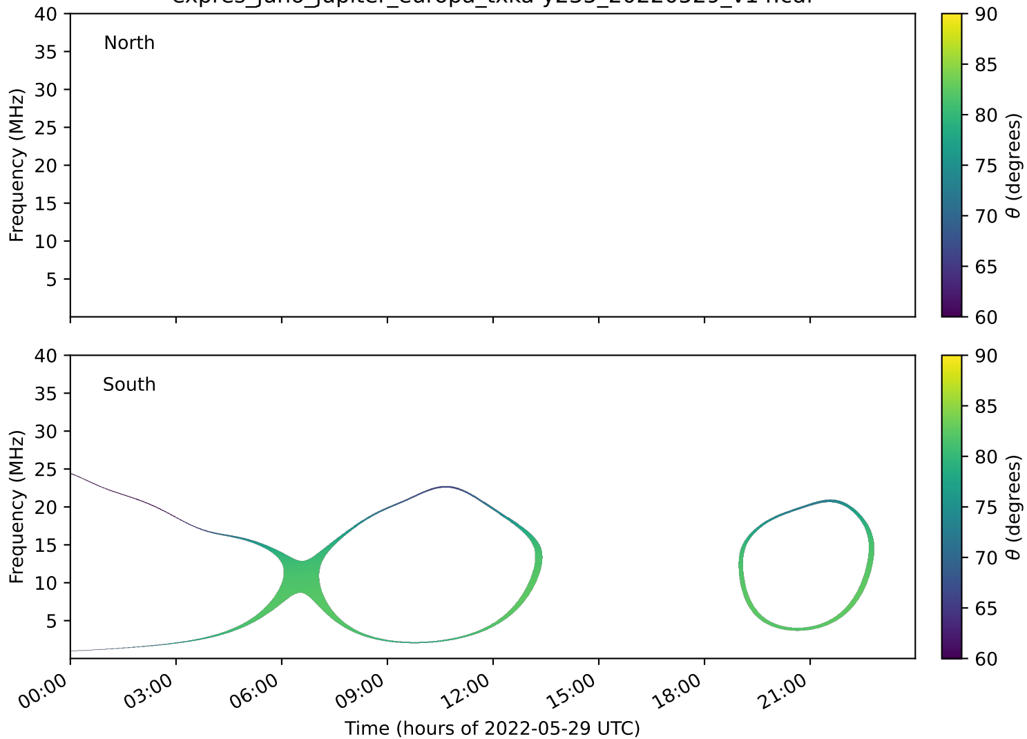
expres_juno_jupiter_europa_txka-y235_20220529_v14.cdf
