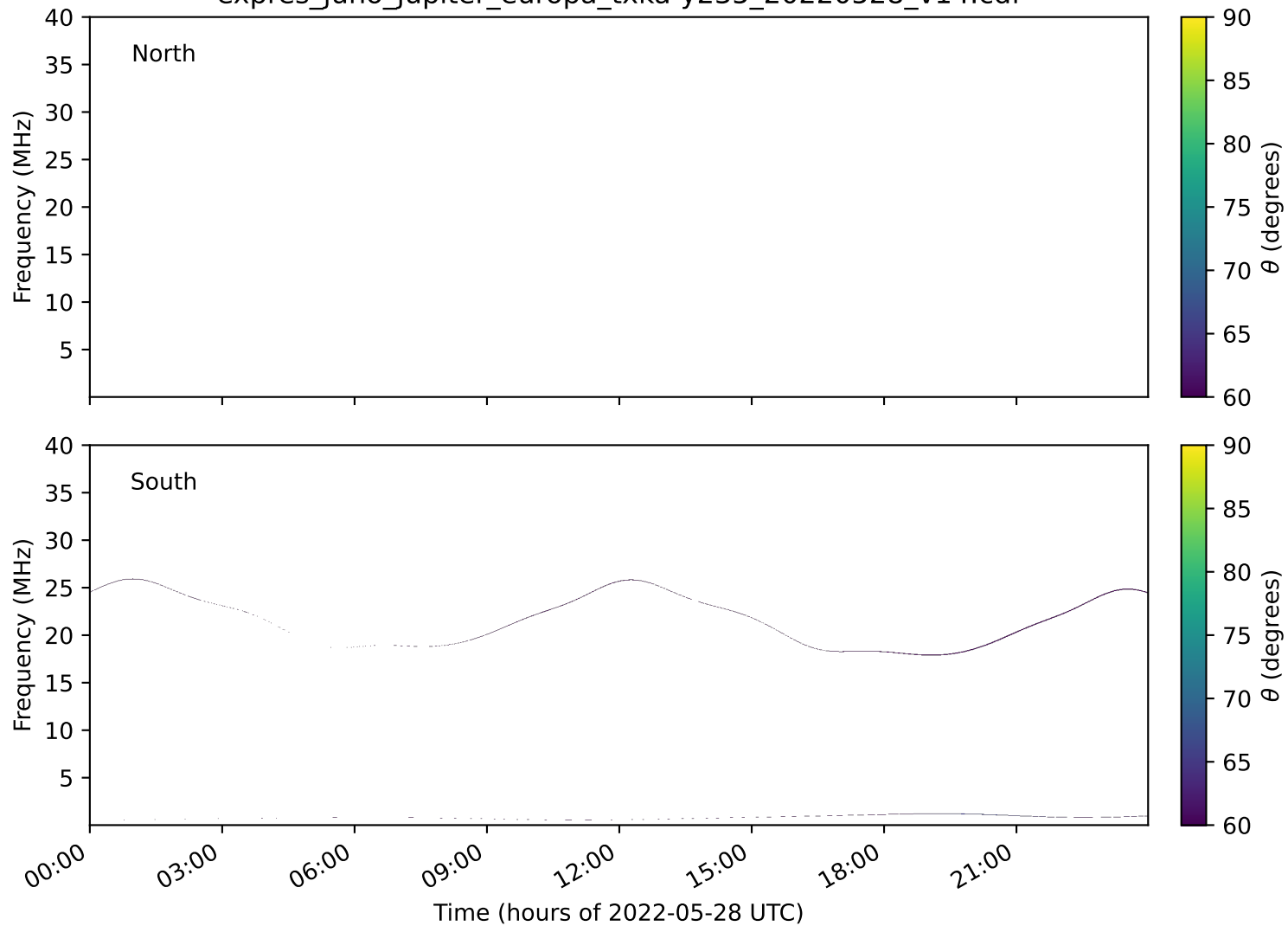
expres_juno_jupiter_europa_txka-y235_20220528_v14.cdf
