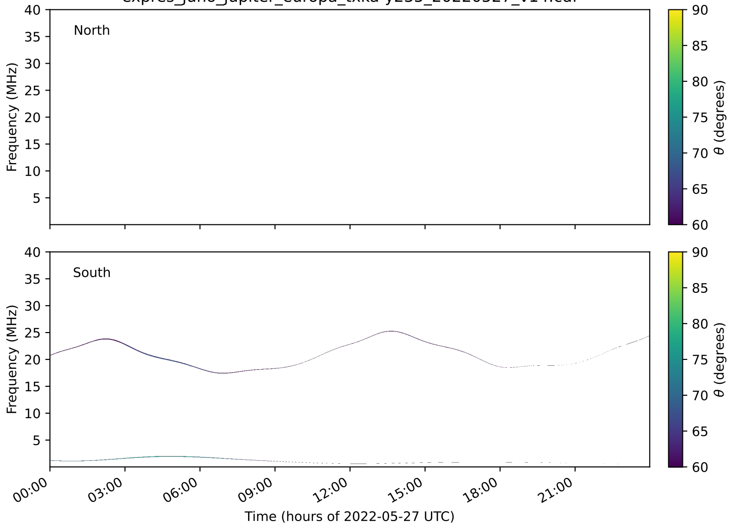
expres_juno_jupiter_europa_txka-y235_20220527_v14.cdf
