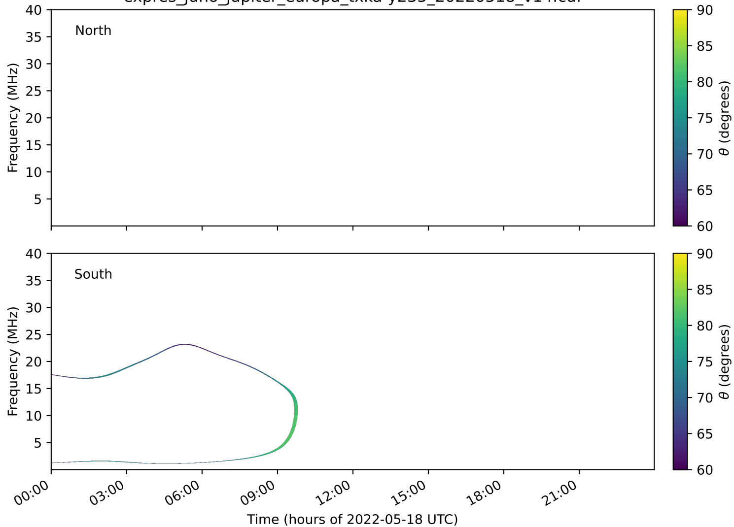
expres_juno_jupiter_europa_txka-y235_20220518_v14.cdf
