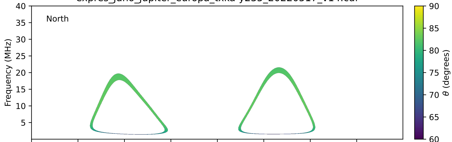
expres_juno_jupiter_europa_txka-y235_20220517_v14.cdf
