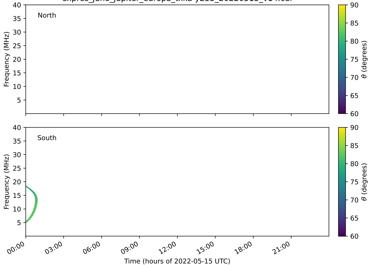
expres_juno_jupiter_europa_txka-y235_20220515_v14.cdf
