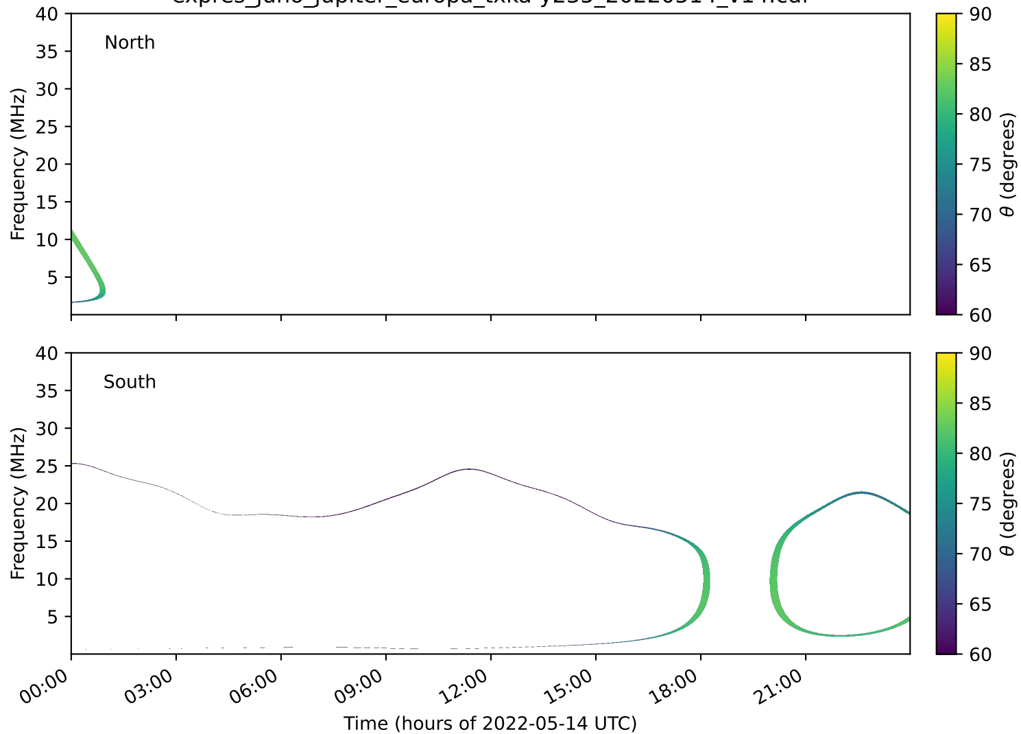
expres_juno_jupiter_europa_txka-y235_20220514_v14.cdf
