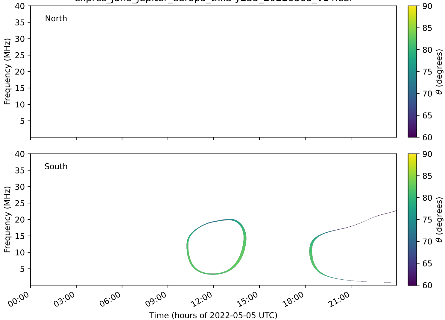
expres_juno_jupiter_europa_txka-y235_20220505_v14.cdf
