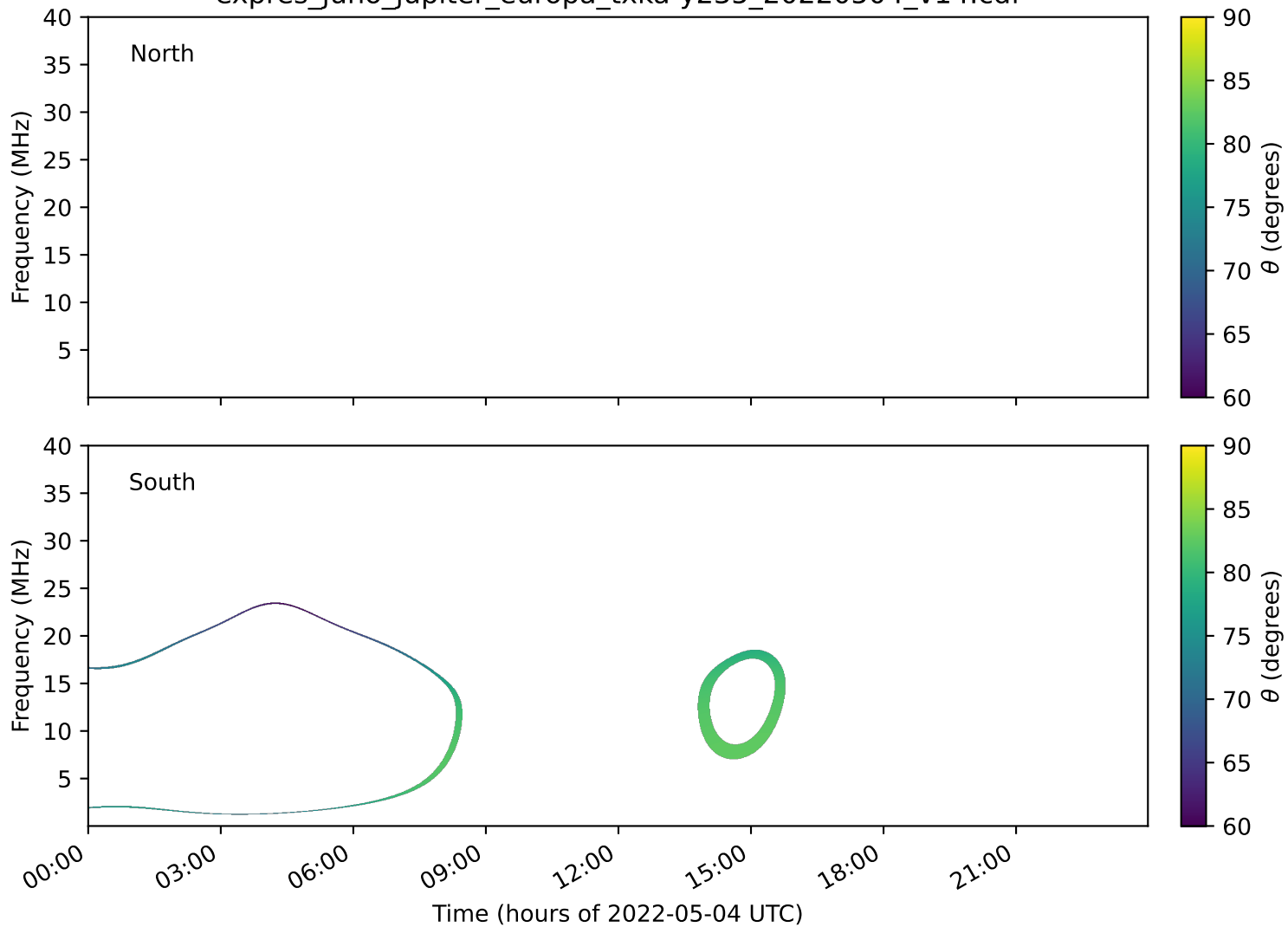
expres_juno_jupiter_europa_txka-y235_20220504_v14.cdf
