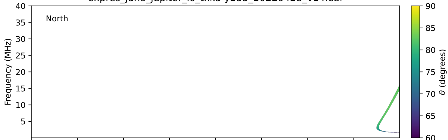
expres_juno_jupiter_io_txka-y235_20220428_v14.cdf
