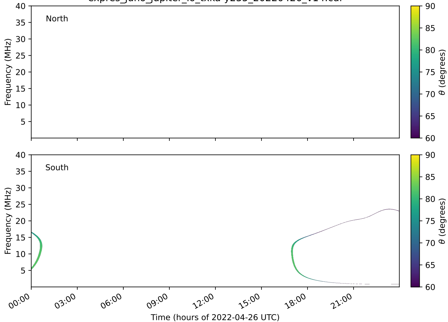
expres_juno_jupiter_io_txka-y235_20220426_v14.cdf
