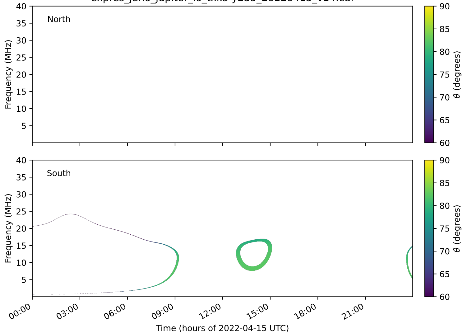
expres_juno_jupiter_io_txka-y235_20220415_v14.cdf
