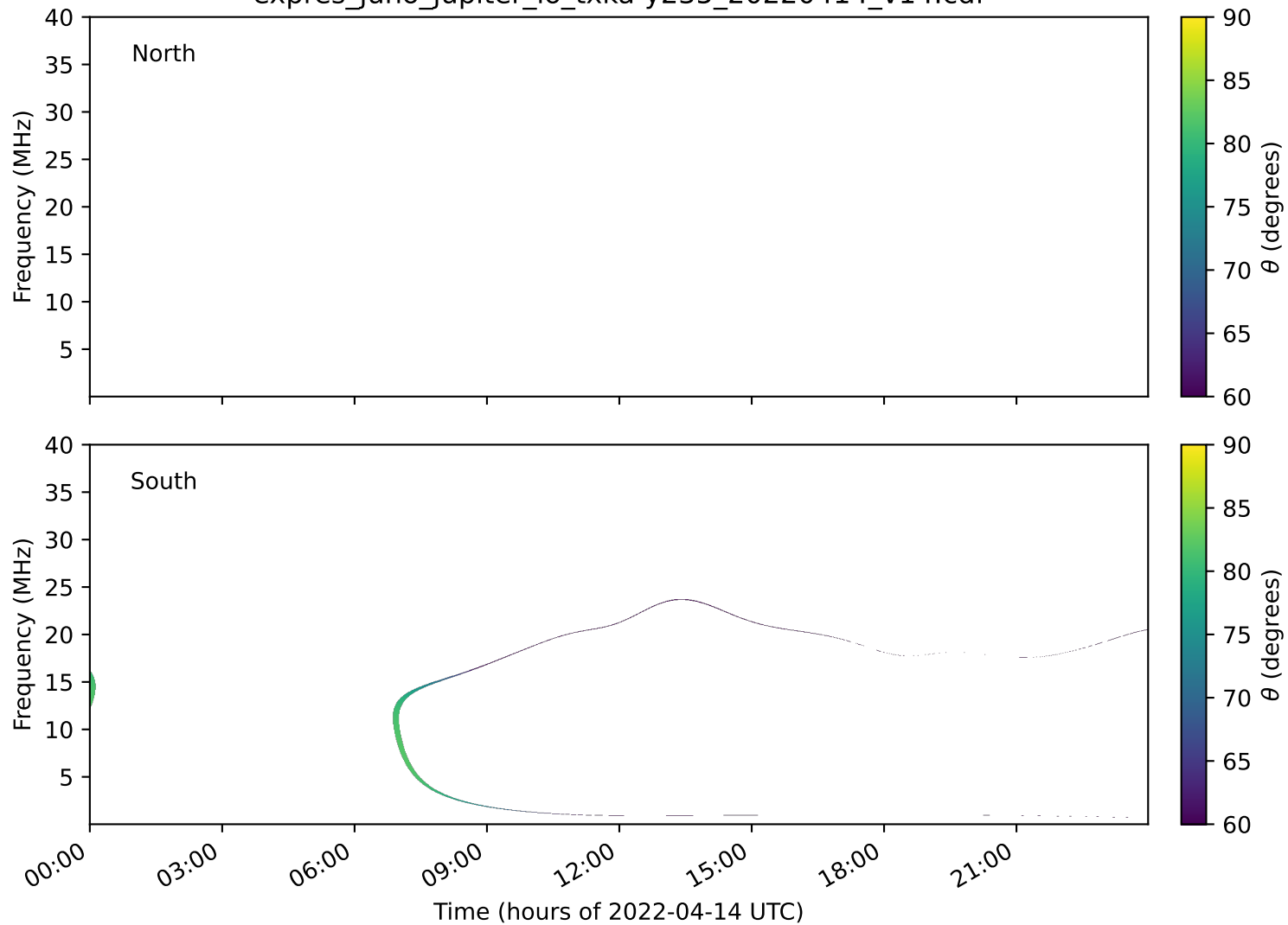
expres_juno_jupiter_io_txka-y235_20220414_v14.cdf
