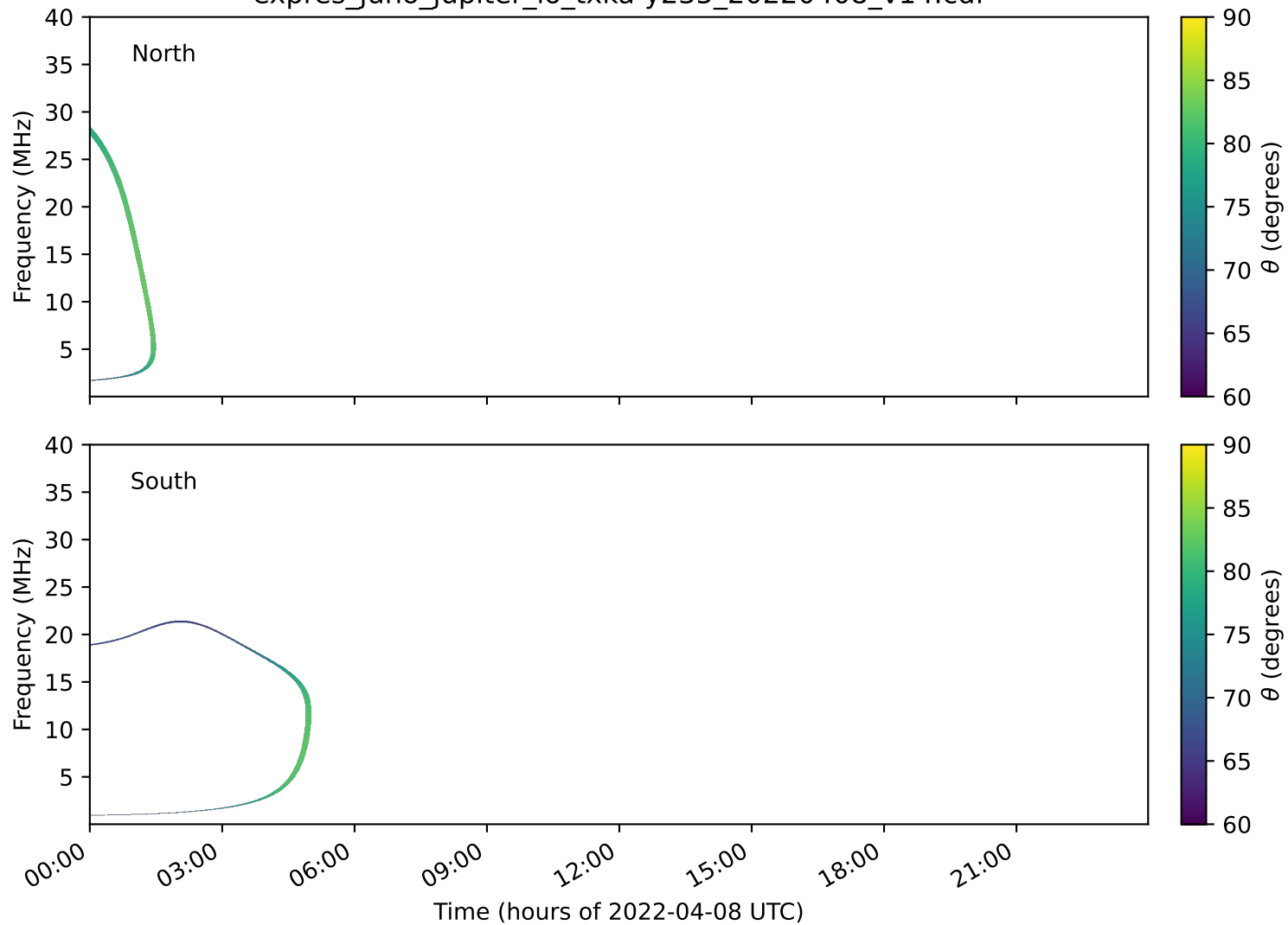
expres_juno_jupiter_io_txka-y235_20220408_v14.cdf
