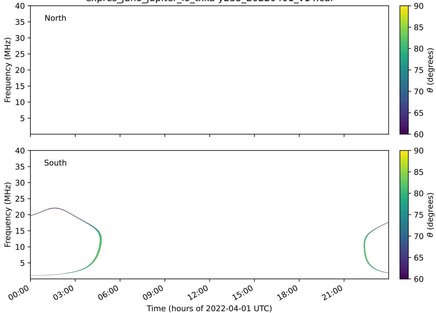
expres_juno_jupiter_io_txka-y235_20220401_v14.cdf
