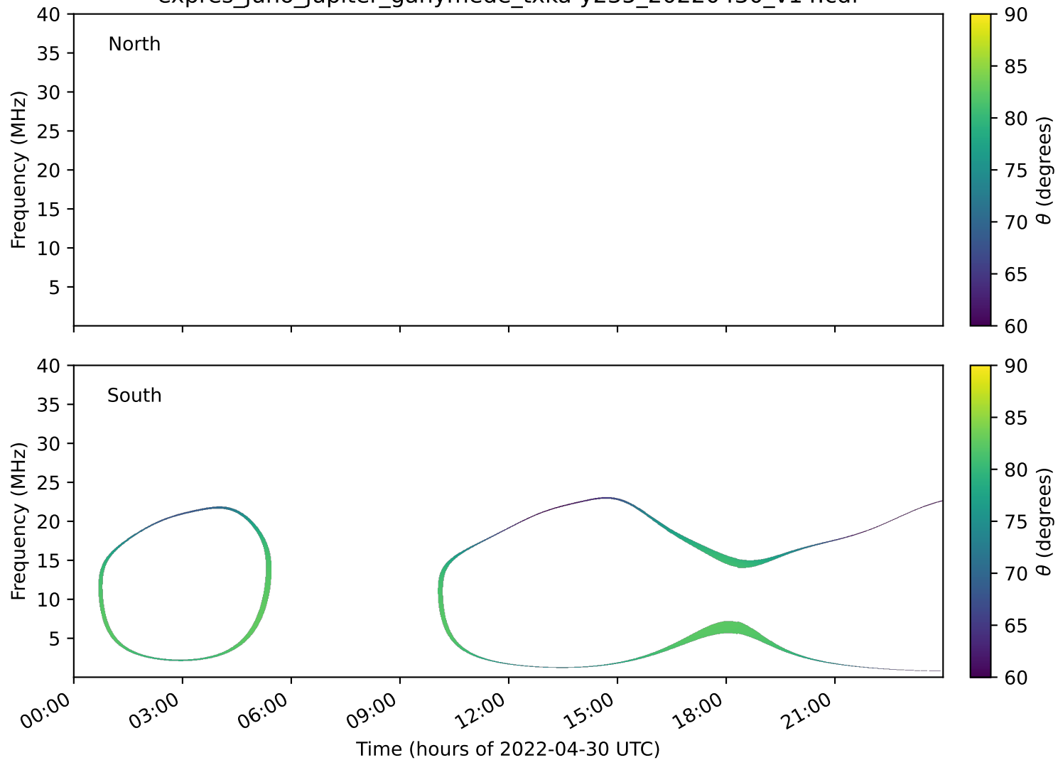
expres_juno_jupiter_ganymede_txka-y235_20220430_v14.cdf
