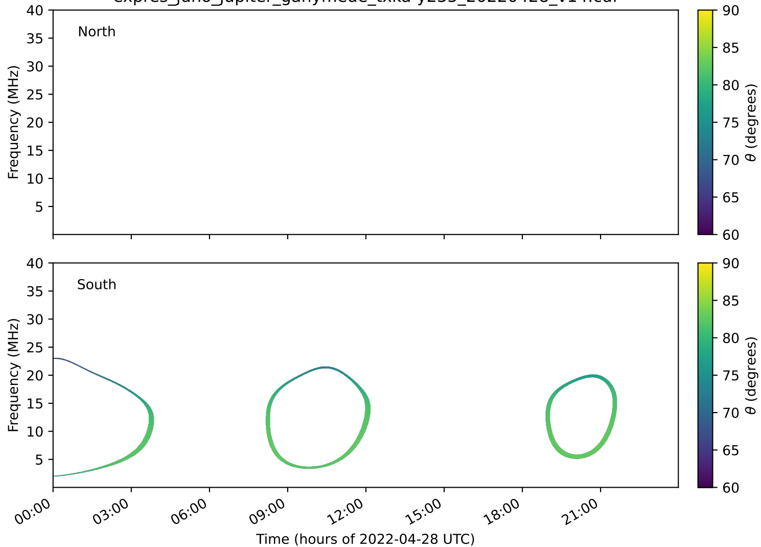
expres_juno_jupiter_ganymede_txka-y235_20220428_v14.cdf
