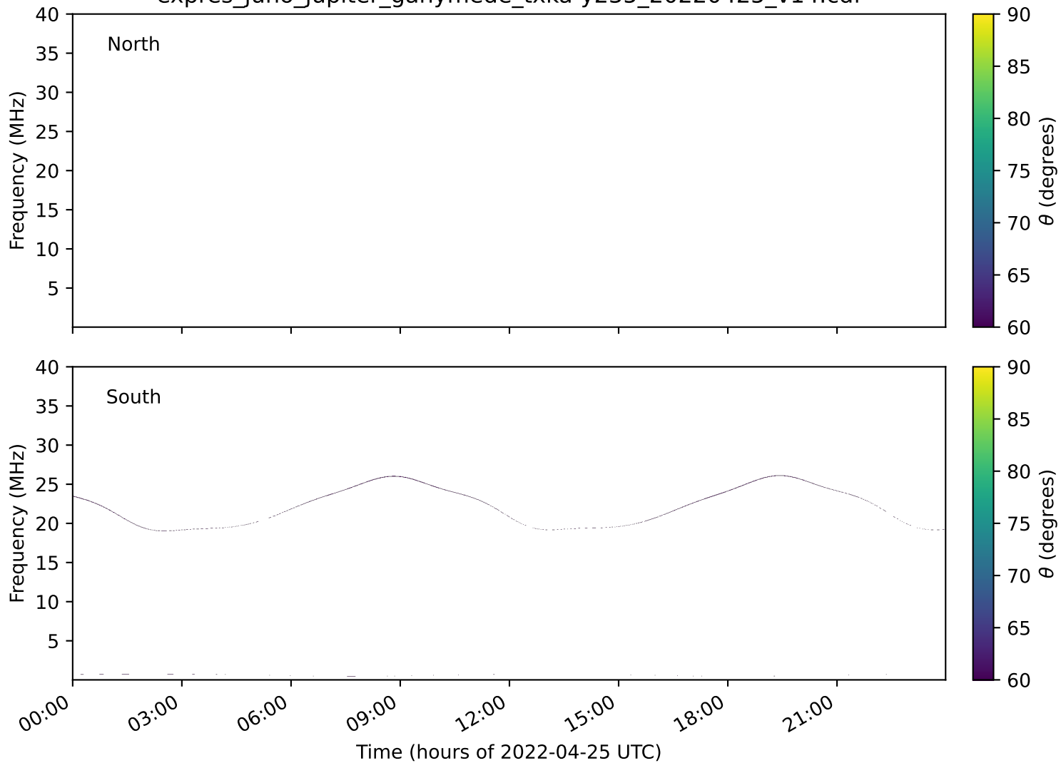
expres_juno_jupiter_ganymede_txka-y235_20220425_v14.cdf
