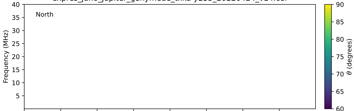
expres_juno_jupiter_ganymede_txka-y235_20220424_v14.cdf
