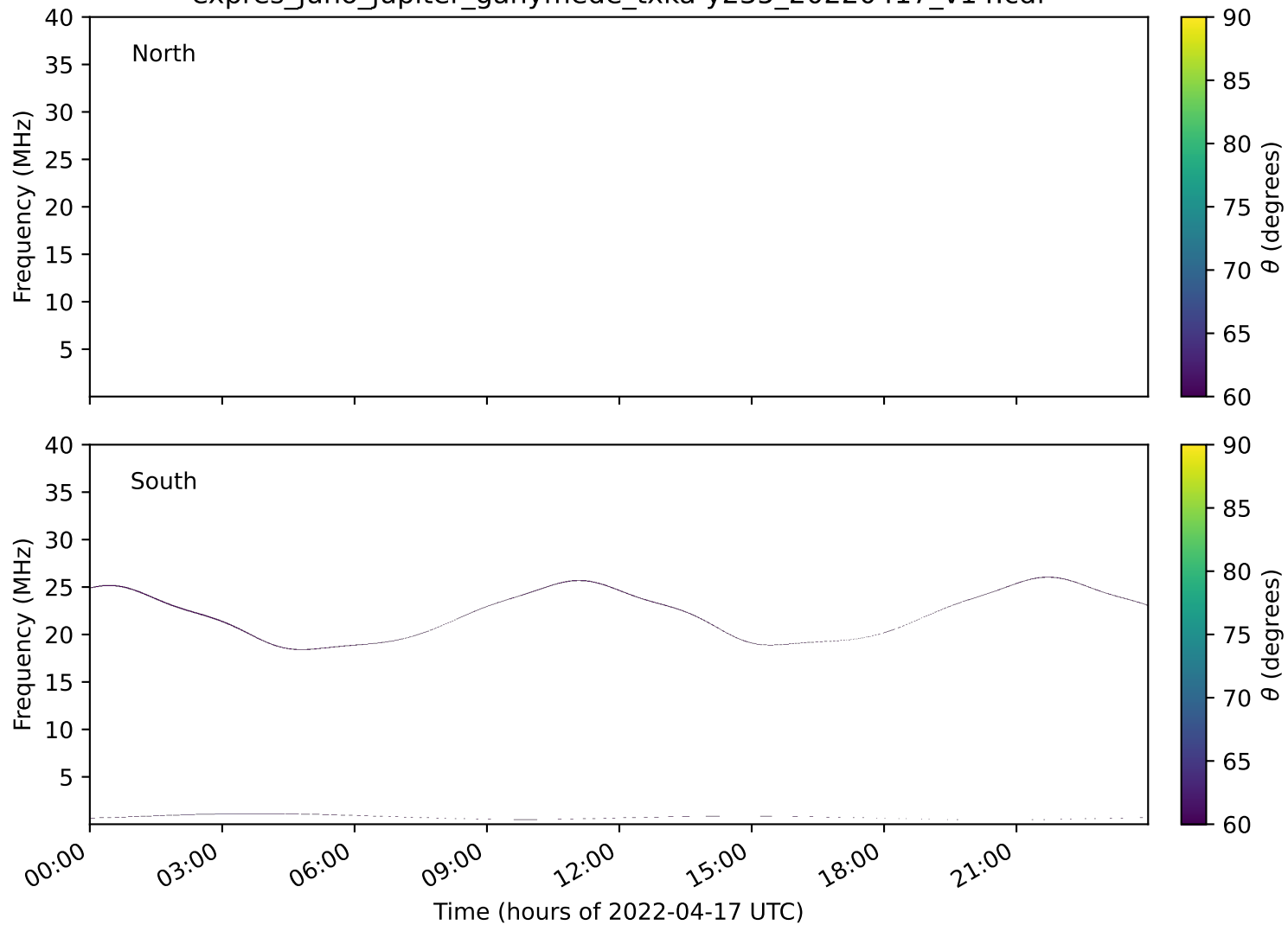
expres_juno_jupiter_ganymede_txka-y235_20220417_v14.cdf
