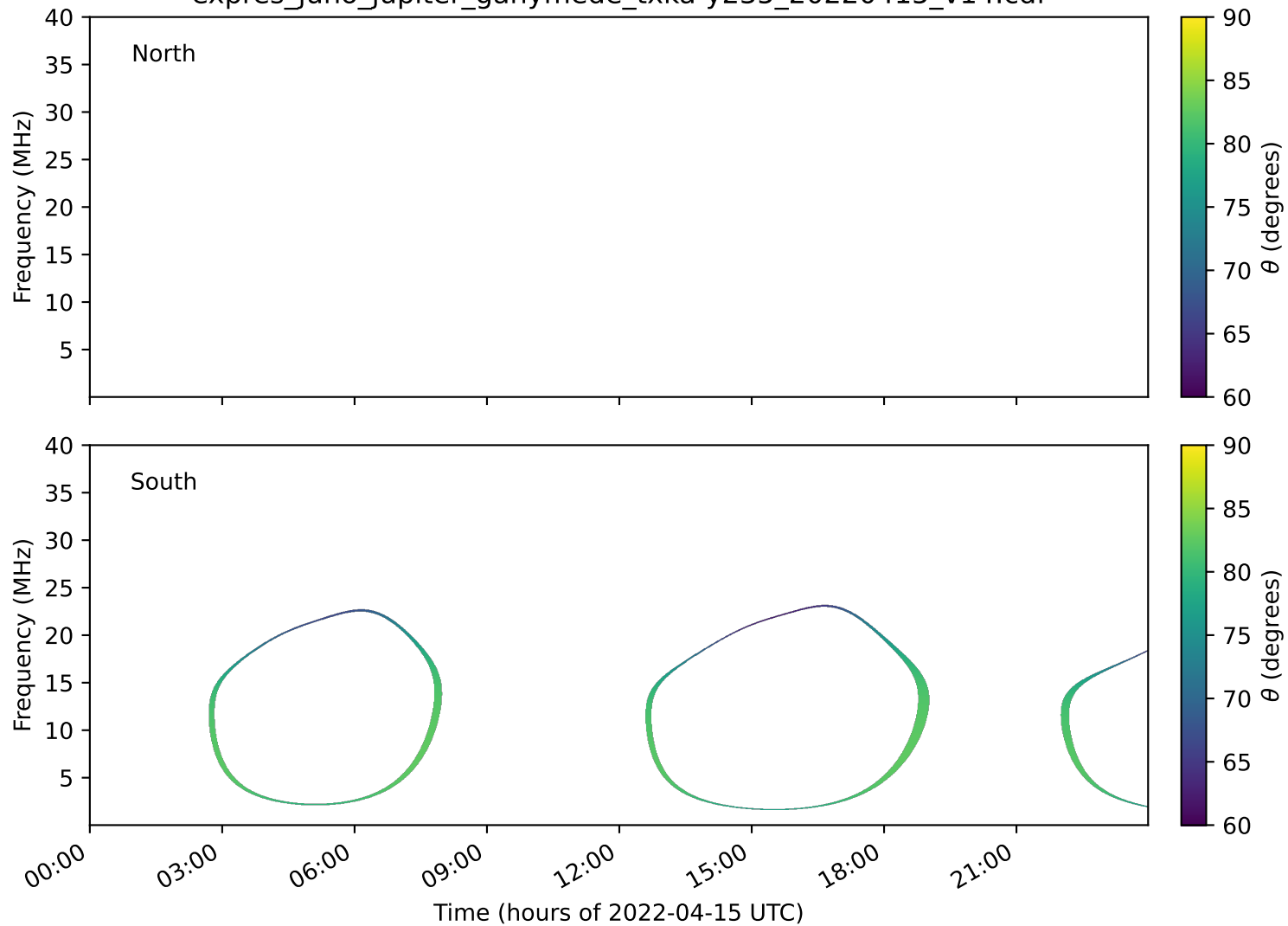
expres_juno_jupiter_ganymede_txka-y235_20220415_v14.cdf
