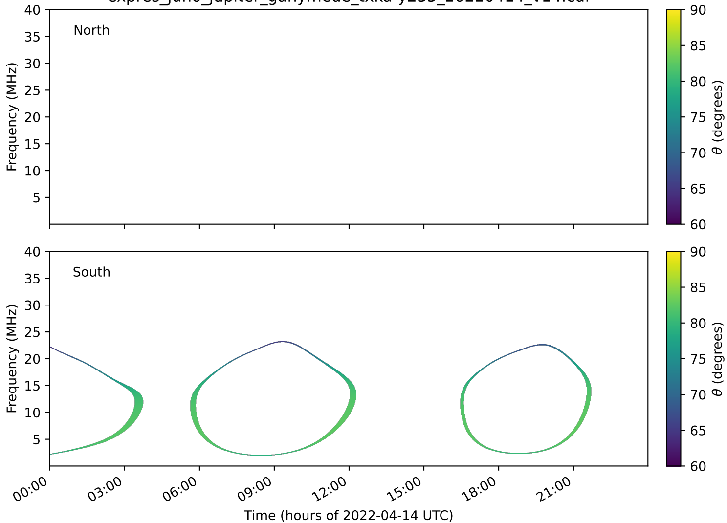
expres_juno_jupiter_ganymede_txka-y235_20220414_v14.cdf
