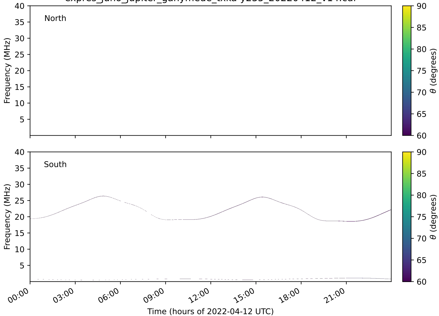
expres_juno_jupiter_ganymede_txka-y235_20220412_v14.cdf
