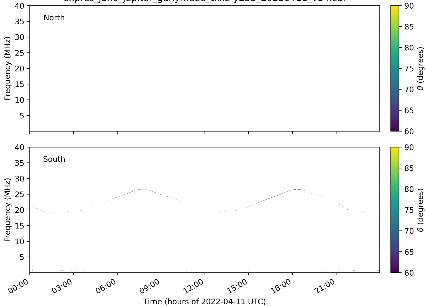
expres_juno_jupiter_ganymede_txka-y235_20220411_v14.cdf
