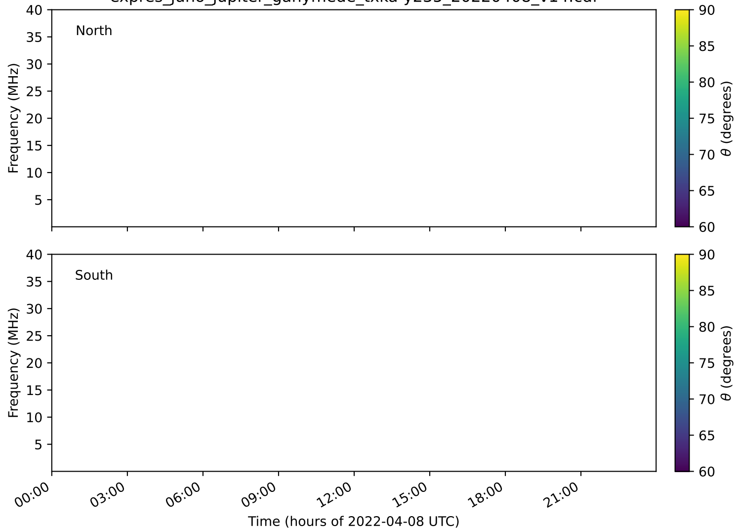
expres_juno_jupiter_ganymede_txka-y235_20220408_v14.cdf
