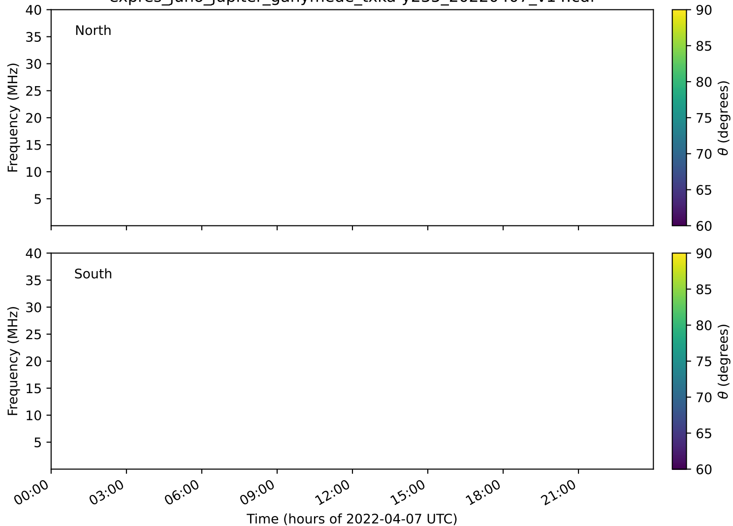
expres_juno_jupiter_ganymede_txka-y235_20220407_v14.cdf
