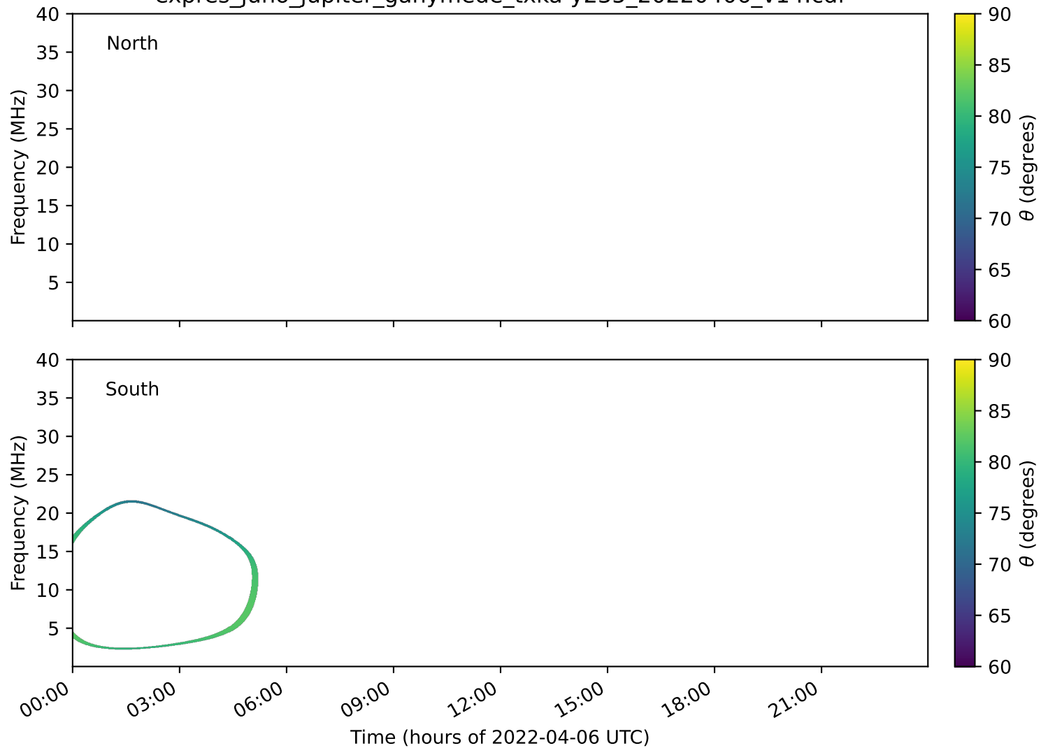
expres_juno_jupiter_ganymede_txka-y235_20220406_v14.cdf
