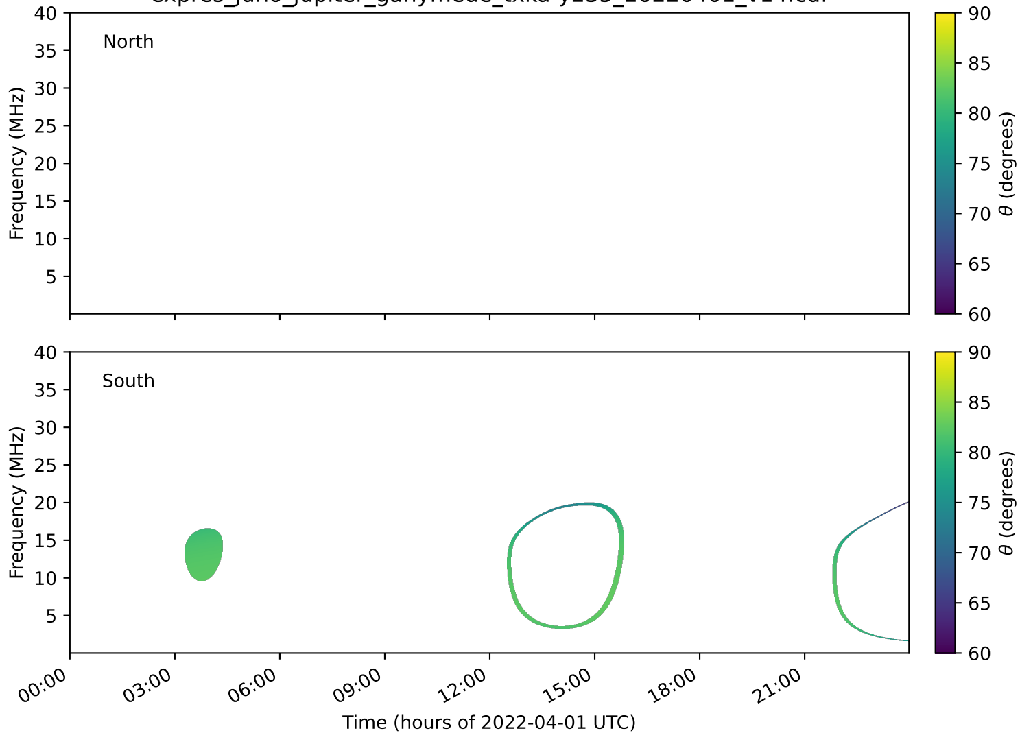
expres_juno_jupiter_ganymede_txka-y235_20220401_v14.cdf
