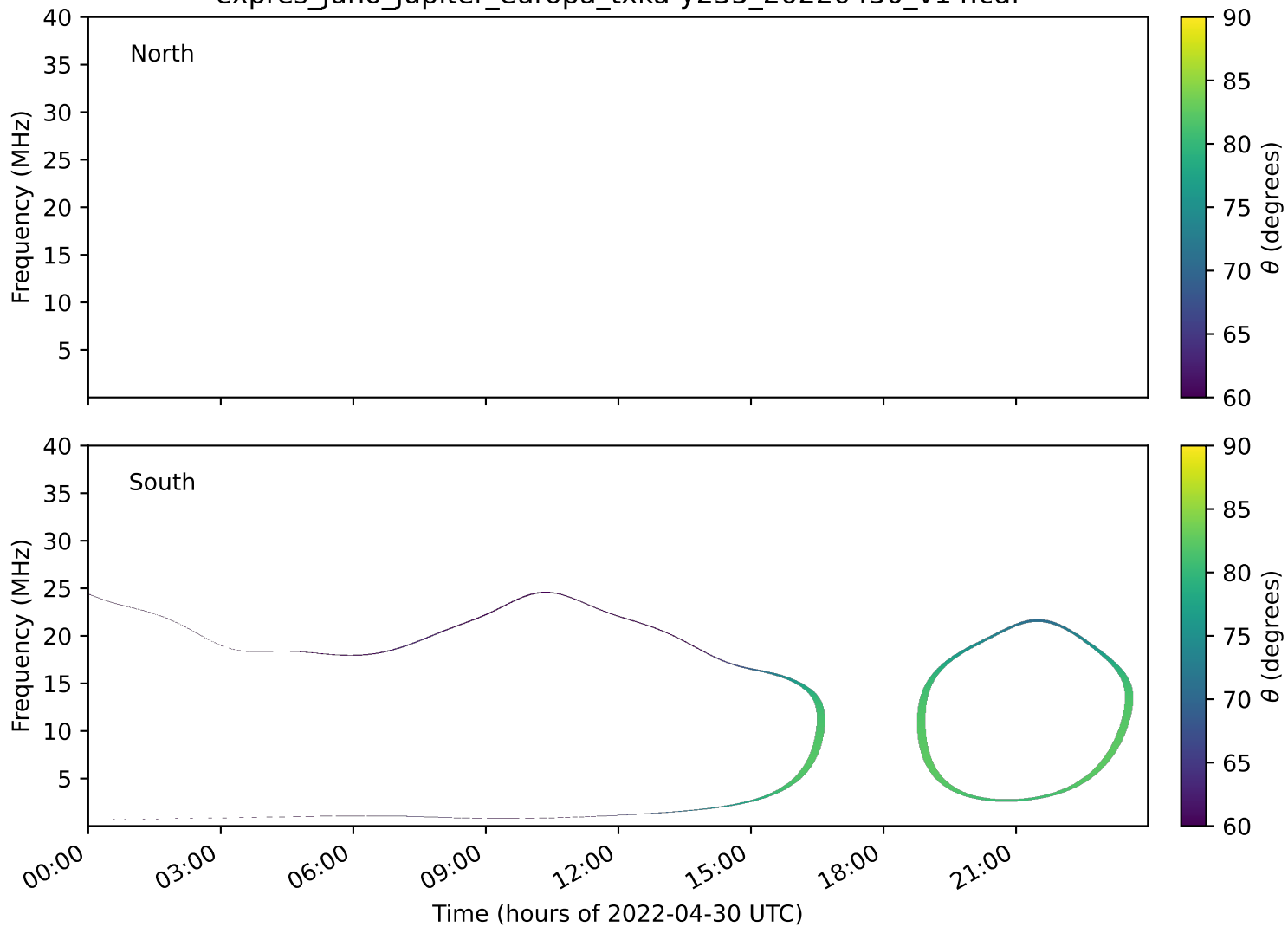
expres_juno_jupiter_europa_txka-y235_20220430_v14.cdf
