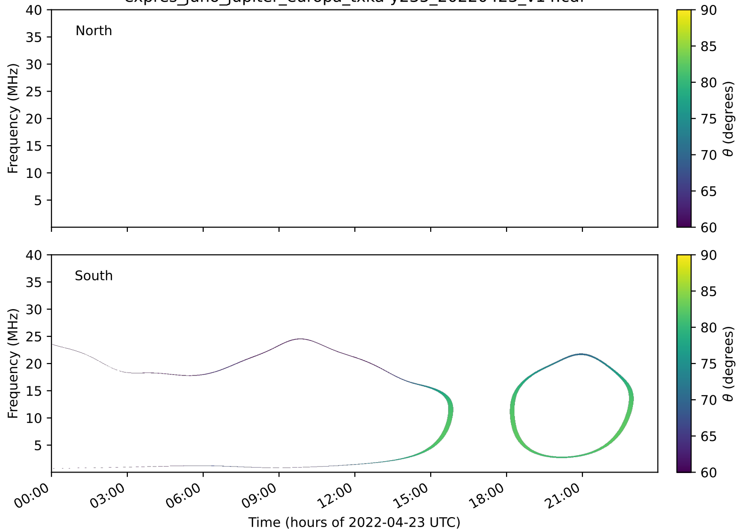
expres_juno_jupiter_europa_txka-y235_20220423_v14.cdf
