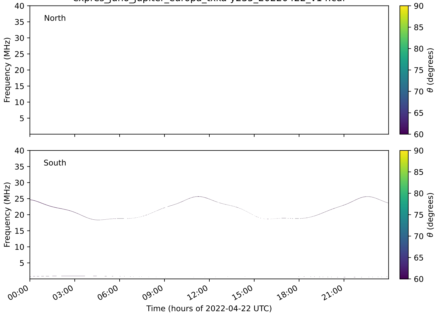
expres_juno_jupiter_europa_txka-y235_20220422_v14.cdf
