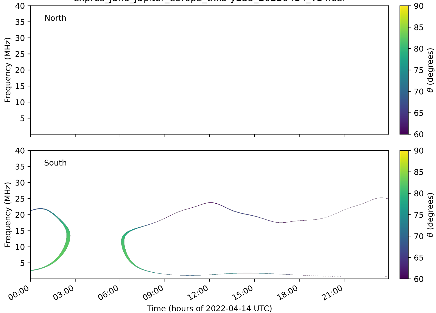
expres_juno_jupiter_europa_txka-y235_20220414_v14.cdf
