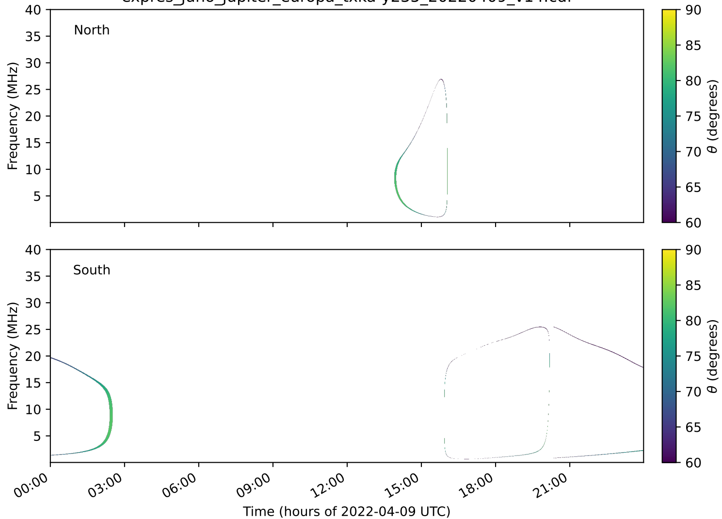
expres_juno_jupiter_europa_txka-y235_20220409_v14.cdf
