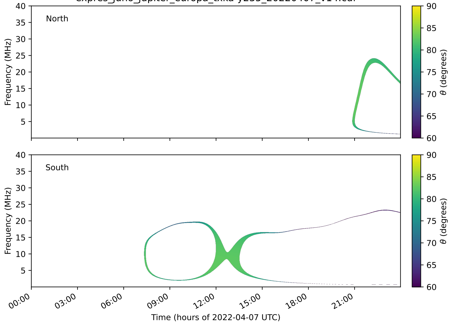
expres_juno_jupiter_europa_txka-y235_20220407_v14.cdf
