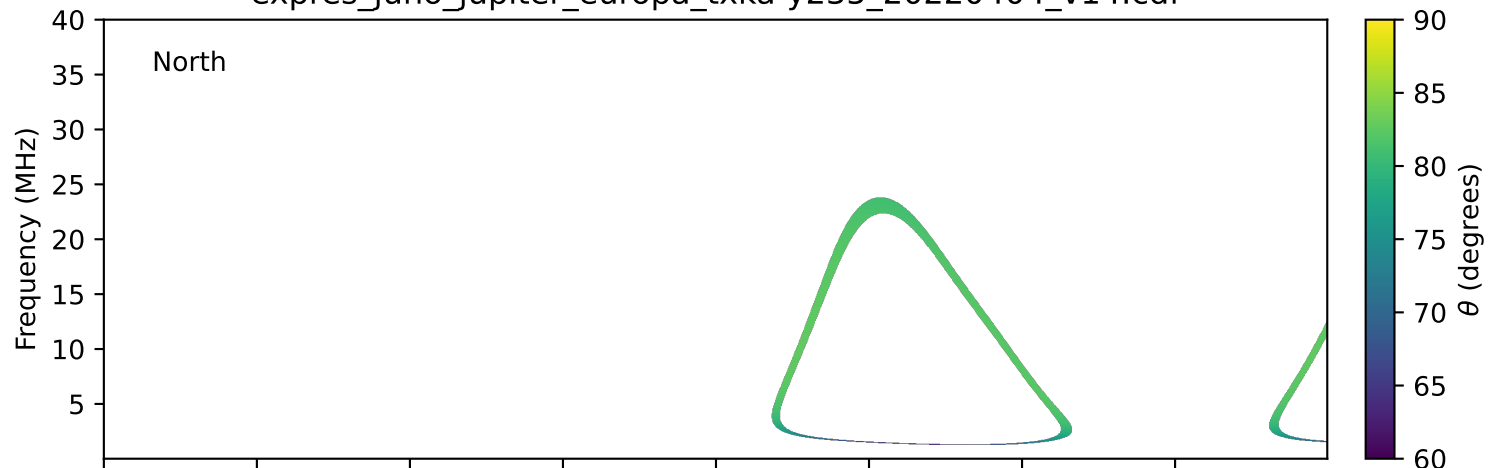
expres_juno_jupiter_europa_txka-y235_20220404_v14.cdf
