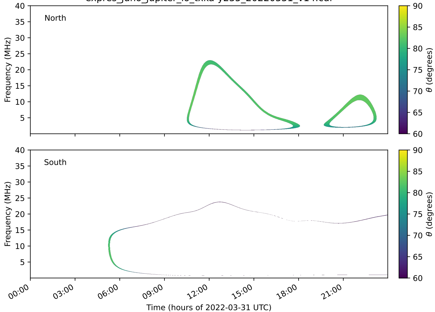
expres_juno_jupiter_io_txka-y235_20220331_v14.cdf
