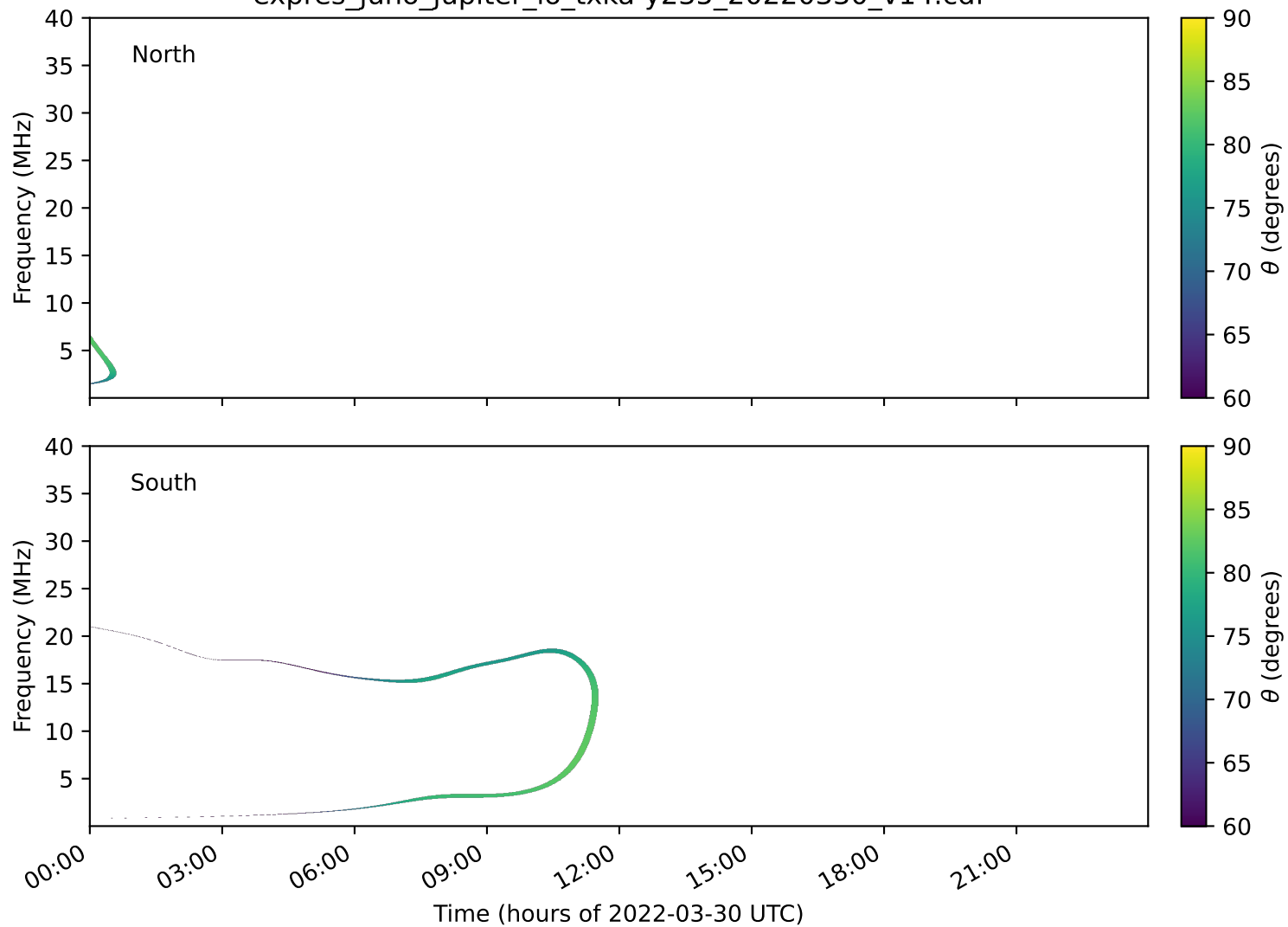
expres_juno_jupiter_io_txka-y235_20220330_v14.cdf
