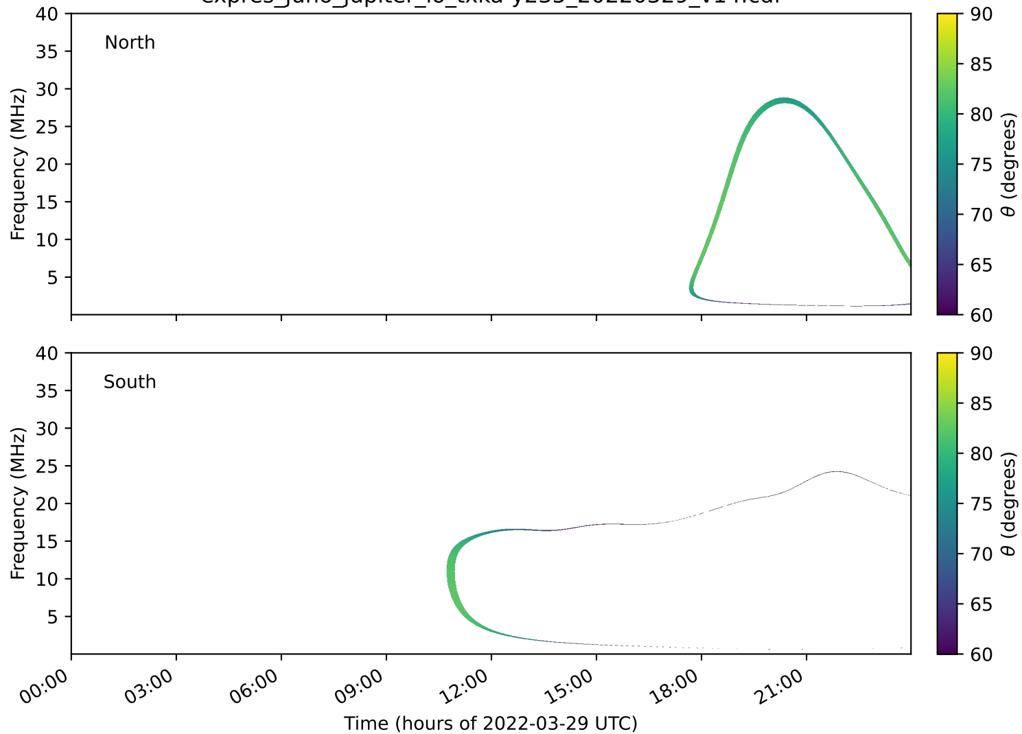
expres_juno_jupiter_io_txka-y235_20220329_v14.cdf
