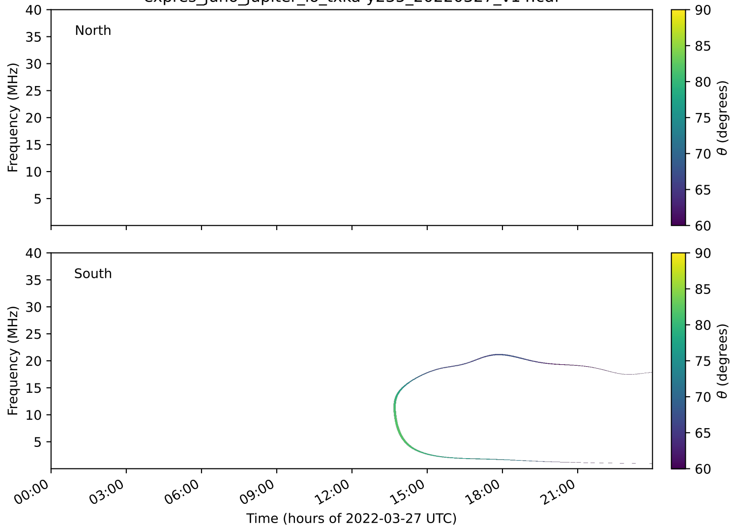
expres_juno_jupiter_io_txka-y235_20220327_v14.cdf
