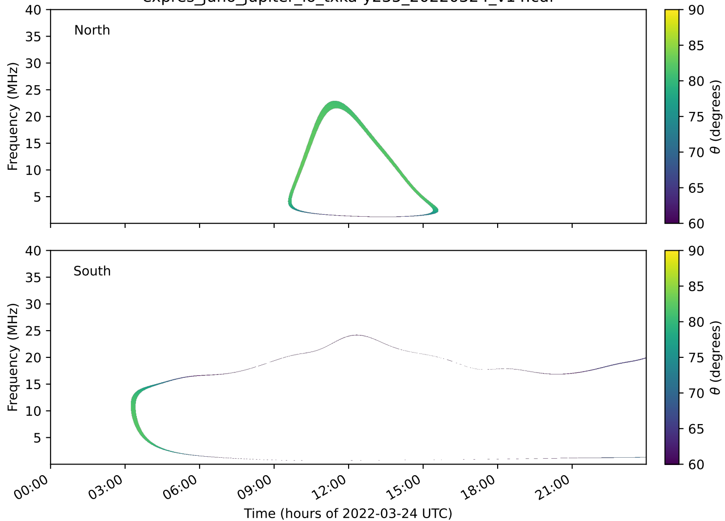
expres_juno_jupiter_io_txka-y235_20220324_v14.cdf
