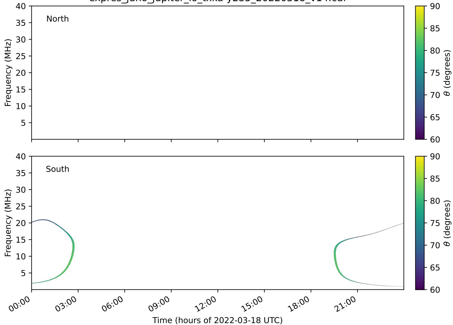
expres_juno_jupiter_io_txka-y235_20220318_v14.cdf
