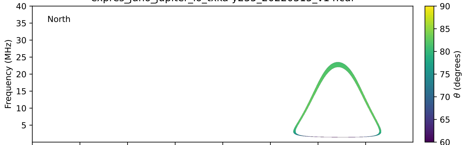
expres_juno_jupiter_io_txka-y235_20220315_v14.cdf
